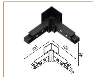
48V-Q2 CONNECTOR HIGH
