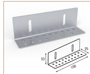
48V-Q2 EMBEDDED BRACKET
