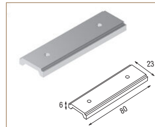
48V-Q2 ALUMINIUM CONNECTION
