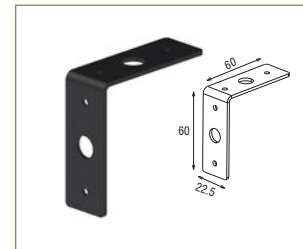
48V-Q2 ANGLE CONNECTION BRACKET
