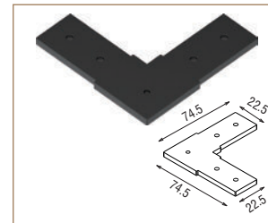
48V-Q2 CONNECTOR SHEET
