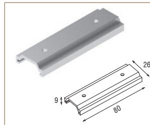
48V-Q1 ALUMINIUM CONNECTION
